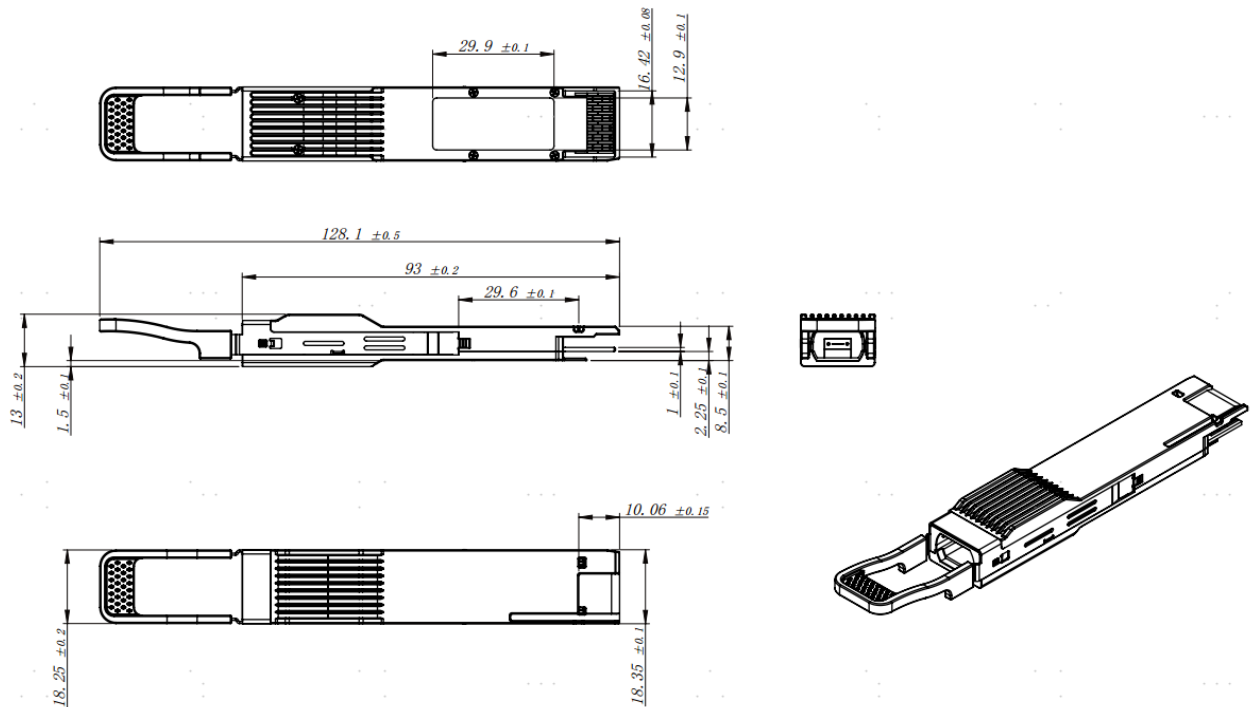
Figure 3. Outline Dimensions
