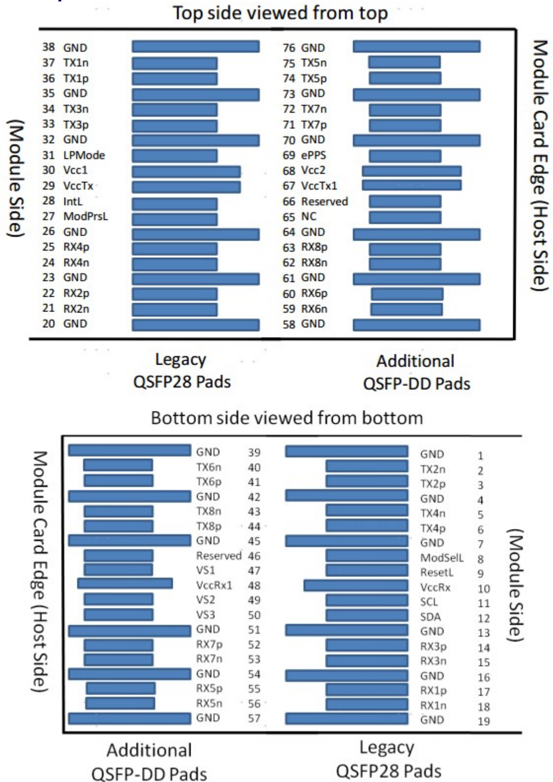
Figure 1. PCB QSFP-DD pad assignment top view
